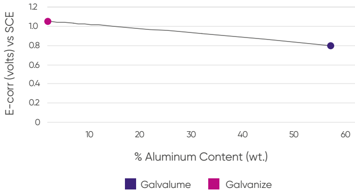
Corrosion Potential After 3 Years Atmospheric Exposure
