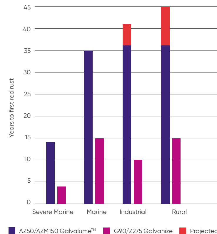
Service Life (years to first red rust)
