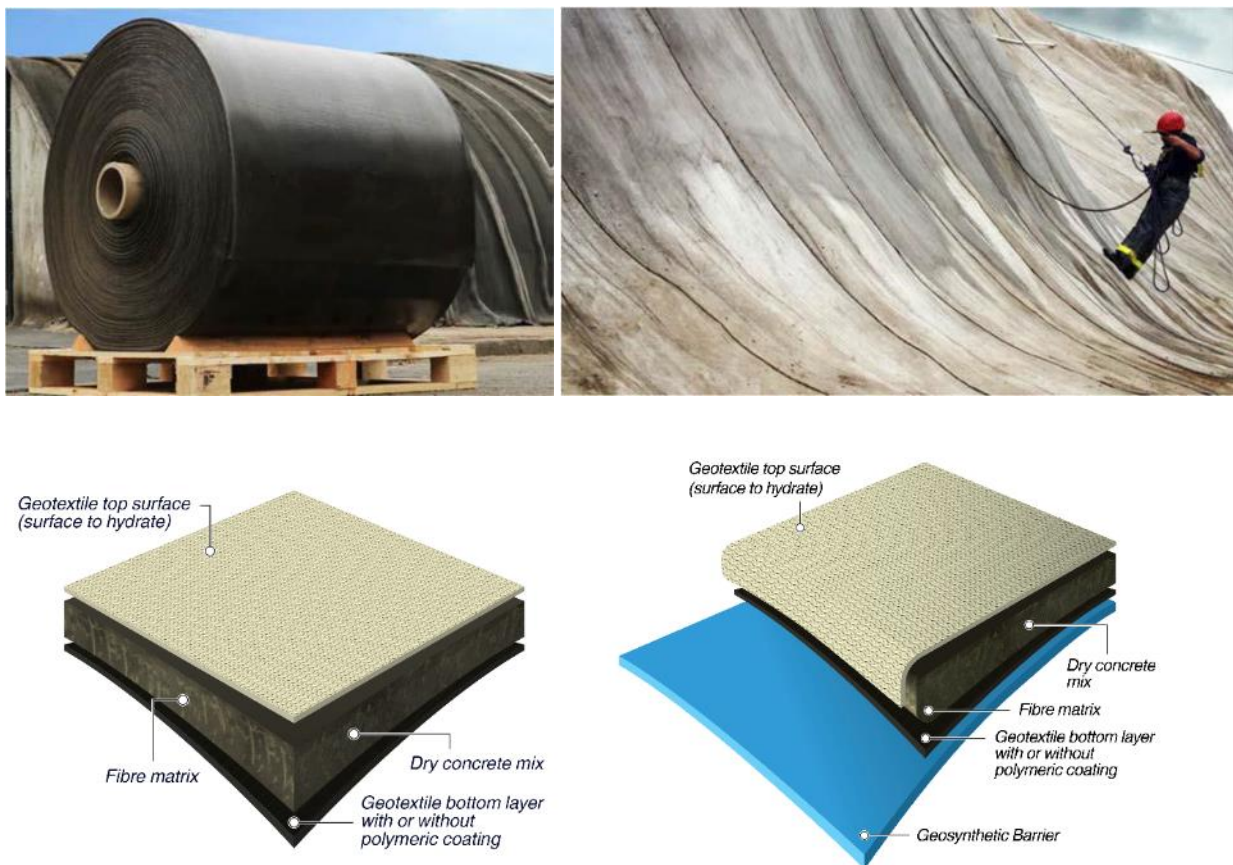
Figure 1.1.1. Geosynthetic Cementitious Composite Mats and Barriers
